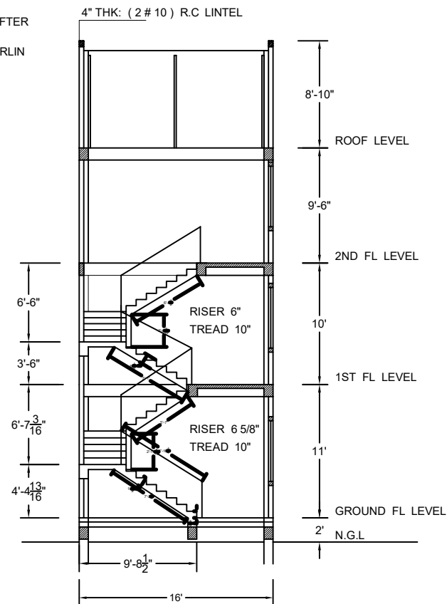
CROSS SECTION
